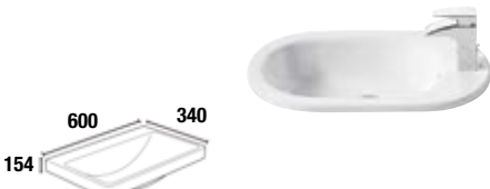
In-countertop Basin
