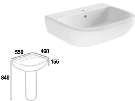
Wash Basin
